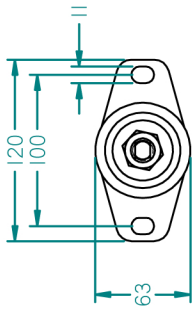
MOUNT DETAILS
